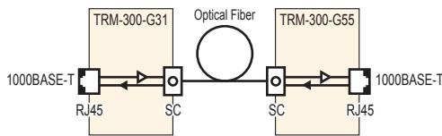
Block Diagram of TRM-300-G31 and TRM-300-G55
