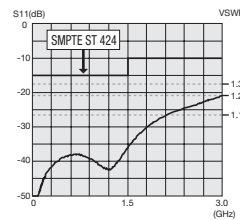
Return loss for BCJ-BPC2P
