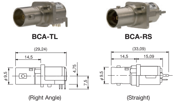
(Right Angle)
