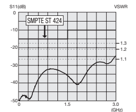
Return loss for MBCP-C3F
