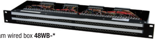
Bantam wired box 48WB-*
