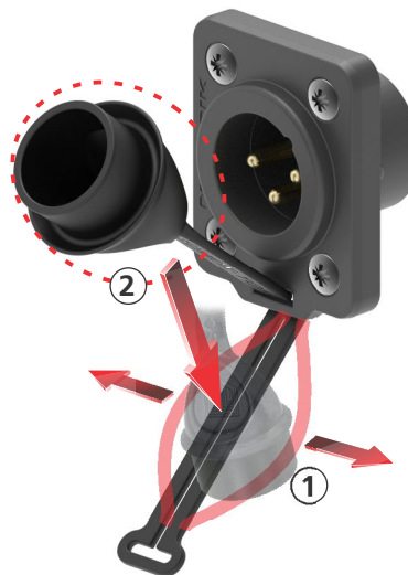
B (1) Split the ribbon and (2) put through the cover.
