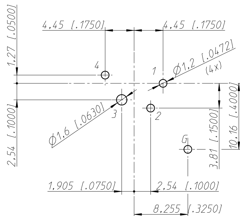
Layout tolerance: ± 0.05 mm [0.002"]
